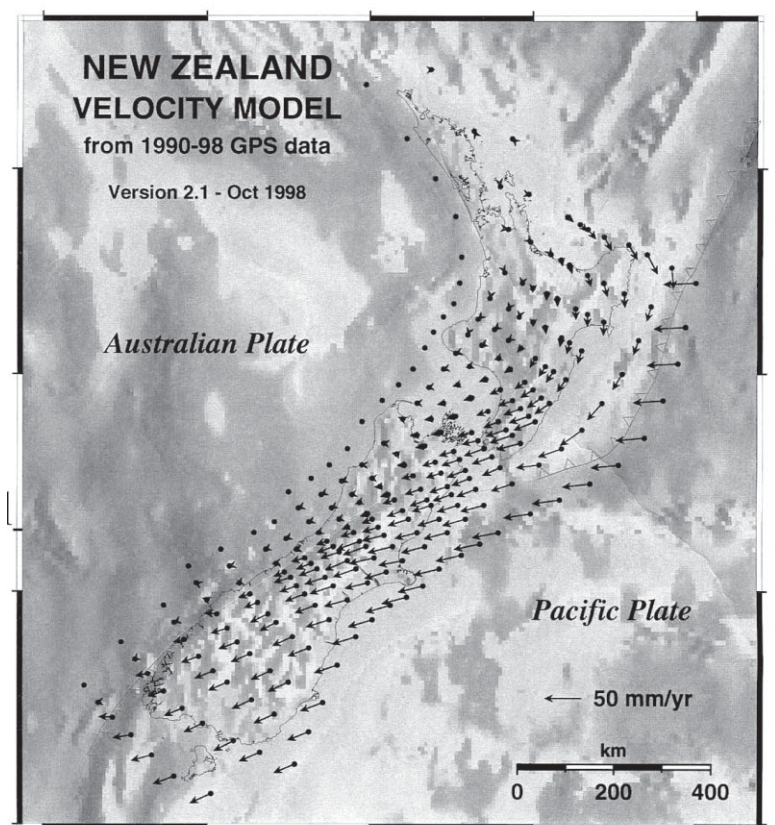
Figure 1. Diagrammatic representation of velocities relative to the Australian plate (developed by the Institute of Geological and Nuclear Sciences)
