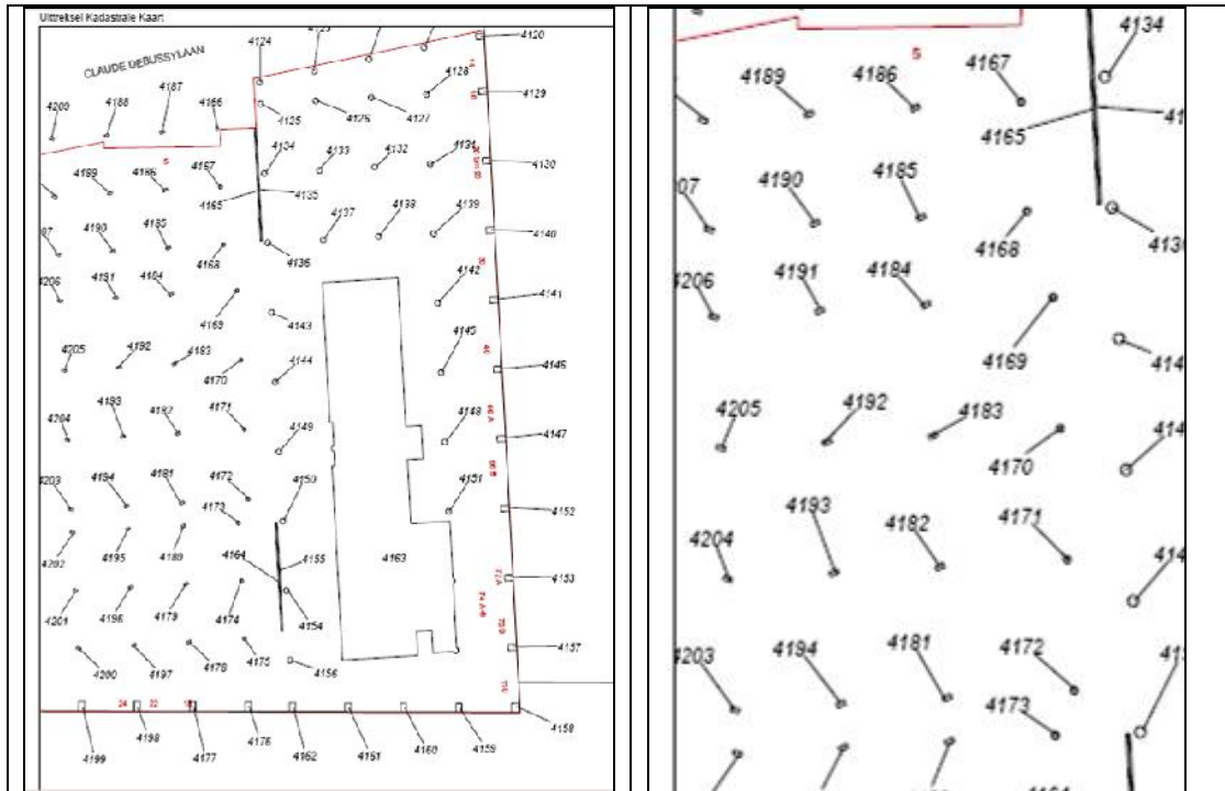
Figure 3: Cadastral map showing the mini-parcels established for the foundation piles of the building in Figure 2
