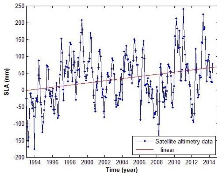
Figure 5. Black Sea level variations from satellite altimetry data.
